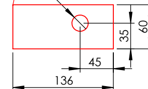
DETAIL E SCALE 1 : 5
