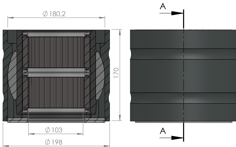
SECTION A-A SCALE 1 : 3.5
