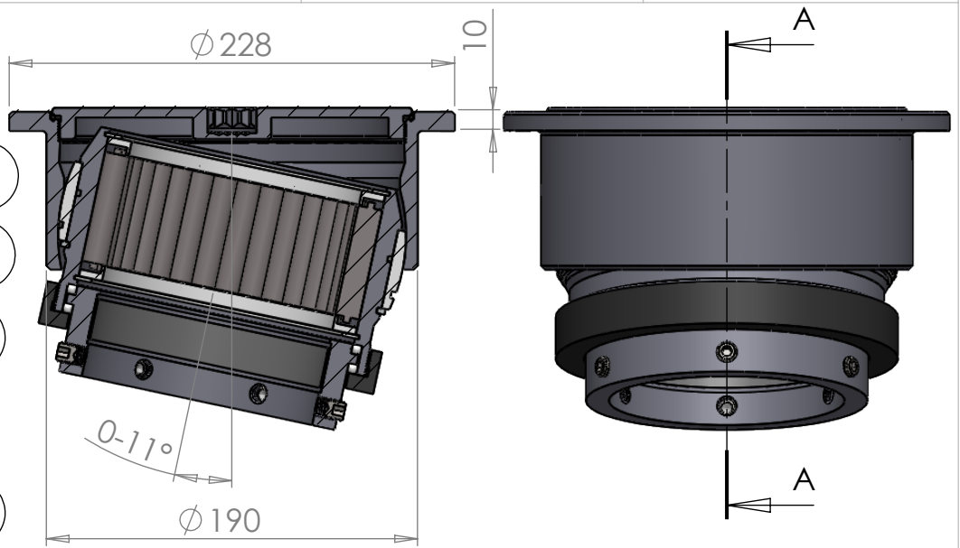
SECTION A-A SCALE 1 : 3.5
