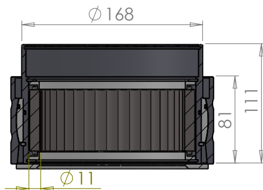
SECTION A-A SCALE 1 : 3.5
