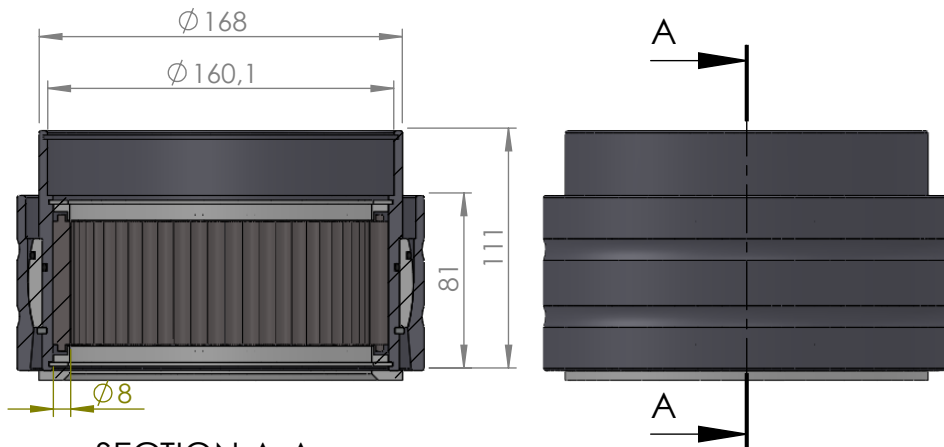
SECTION A-A SCALE 1 : 3.5
