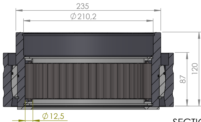
SECTION A-A SCALE 1 : 3.5
