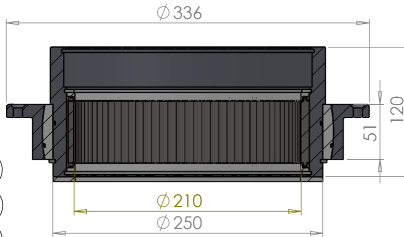
SECTION A-A SCALE 1 : 3.5
