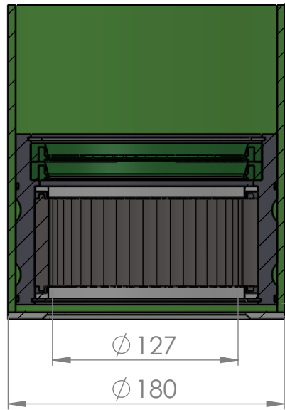
SECTION A-A SCALE 1 : 3.5
