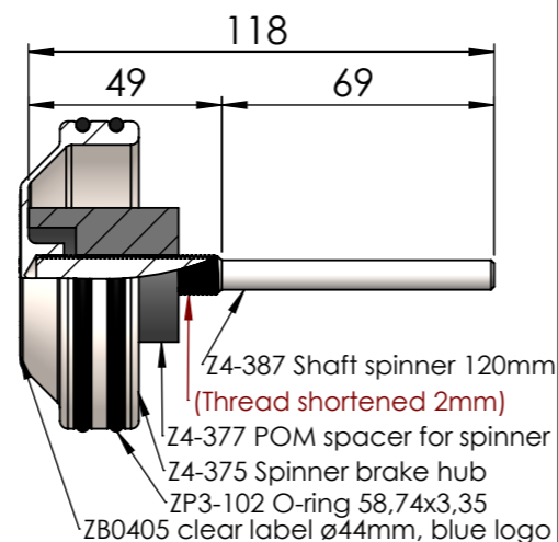
SP-SP150 carbon wheel big cone BS25
