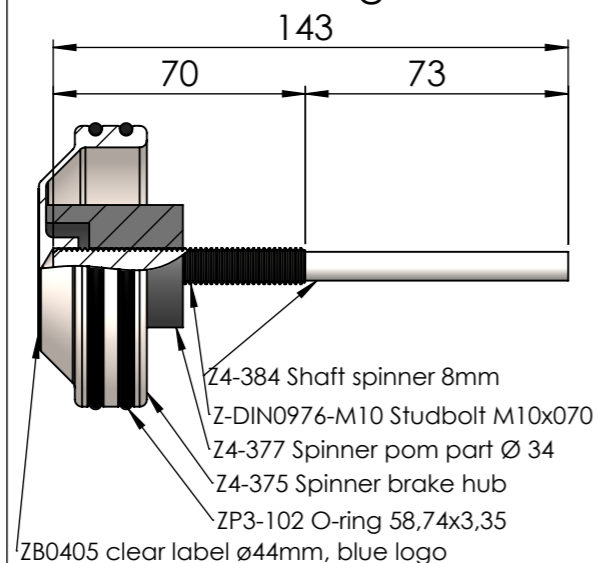
SP-SP143 carbon wheel big cone BS30
